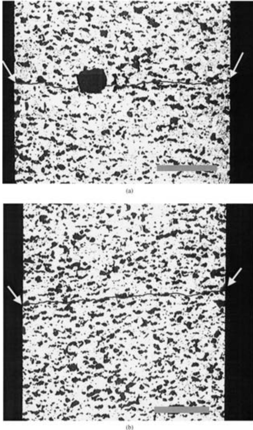
Figure 5 Specimen surfaces with fracture lines after test (between arrows). The bar equals 1 mm. a) huge surface pore could be identified as fracture origin (upper picture), b) surface and volume pores could not be distinguished as fracture origin (lower picture).
